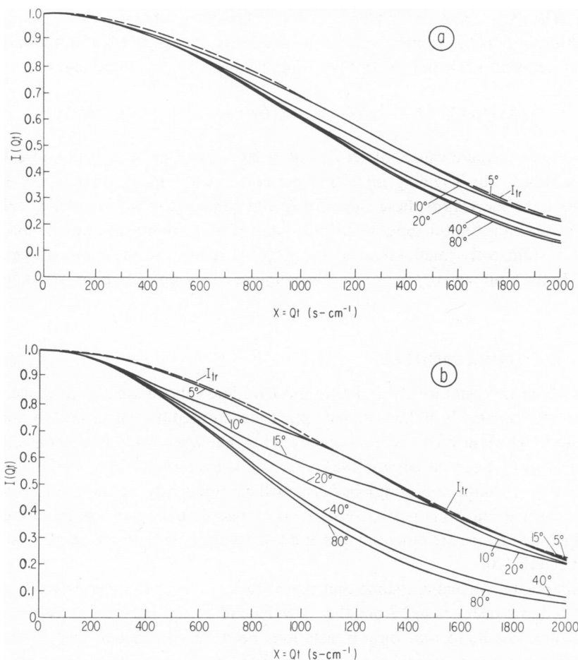
FIGURE 5 Normalized intensity correlation function I_{\text{lin}}^w(Q, t) for a distributed line of scattering centers (see Eq. 29). Here, b_1 = 0 , b_2 = 1 \mu\text{m} , \langle V^2 \rangle^{1/2} = 15 \mu\text{m/s} , A = 30^\circ . (a) \nu = \omega_0/2\pi = 5 \text{ s}^{-1} . (b) \nu = 10 \text{ s}^{-1} . The precise values of the parameters are unimportant; for example, we could have taken b_2 = 1.8 \mu\text{m} , A = 25^\circ , \nu = 3.3 \text{ s}^{-1} and have obtained essentially the same curves as those given in Fig. 5 a. Note, also, the similarity between the expression used to compute these curves and those given in Eqs. 31 and 32.
