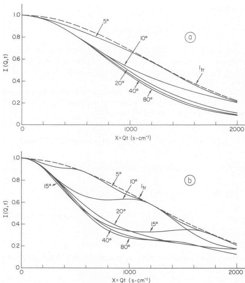
FIGURE 4 Normalized intensity correlation functions I_{db}^w(Q, t) , for motile two-point dumbbells which are wiggling, calculated according to Eqs. 1 and 26 for different scattering angles. (a) Parameters: distance between centers d = 1.5 \mu\text{m} , mean translational speed \langle v^2 \rangle^{1/2} = 15 \mu\text{m/s} , maximum wiggle angle A = 30^\circ , wiggle frequency \nu = \omega_0/2\pi = 5 \text{ s}^{-1} ; (b) same parameters as (a), except that \nu = 10 \text{ s}^{-1} .
